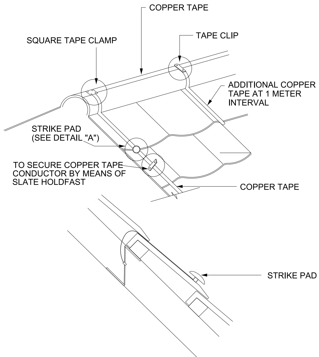
DETAIL "A": STRIKE PAD
